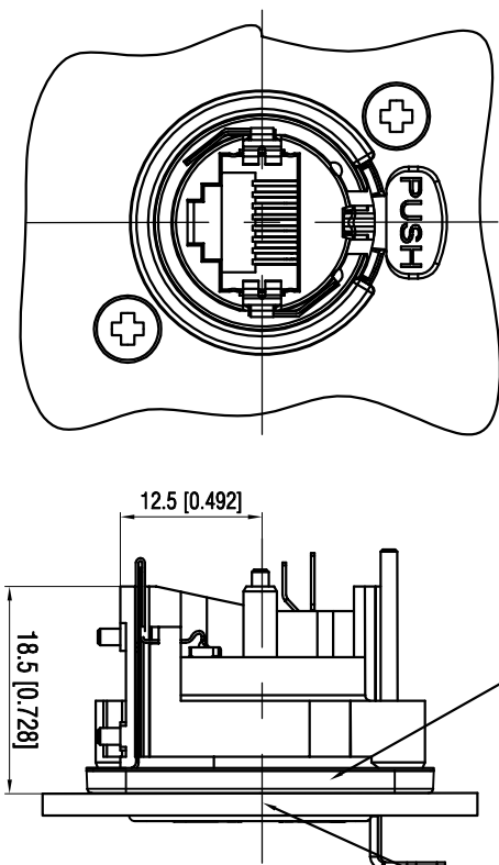
Flange fixed on the inside of the panel
