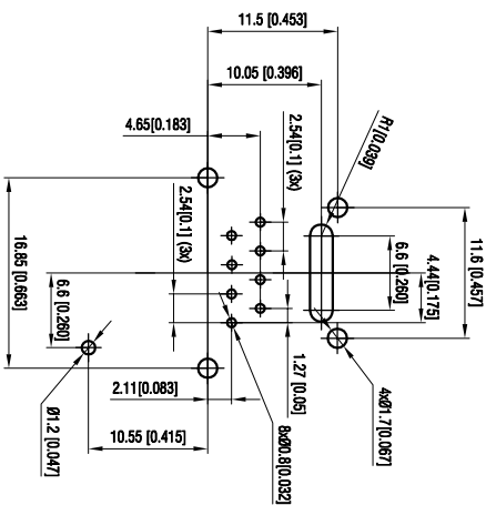
PCB Layout (Scale 2:1)
