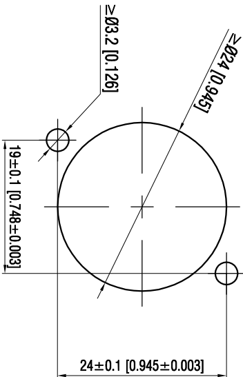
Panel Cut out dimension
